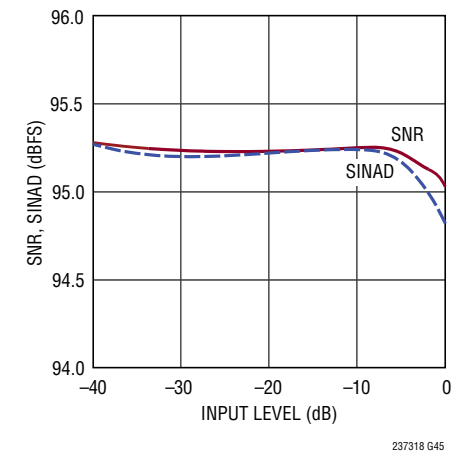
SNR, SINAD vs Input Level, f_{IN} = 1\text{kHz}
